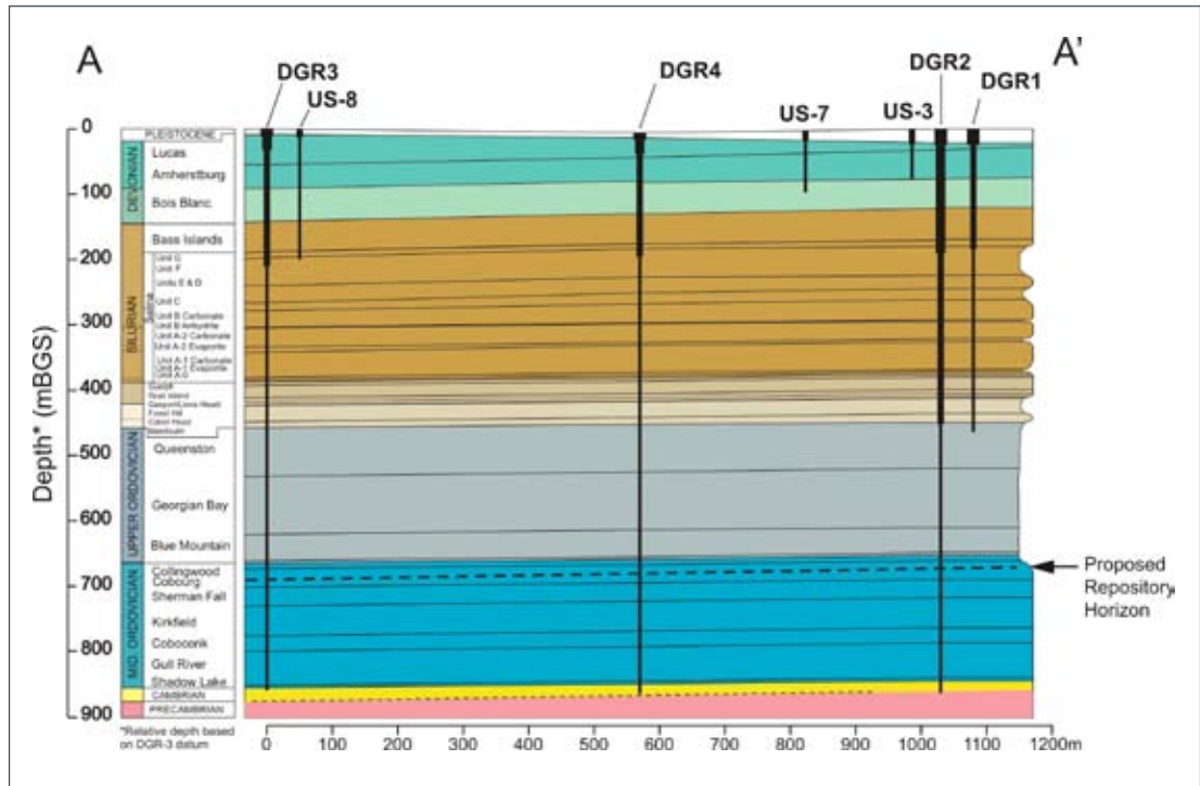
Geologic cross-section showing bedrock formations/stratigraphy beneath the Bruce nuclear site
