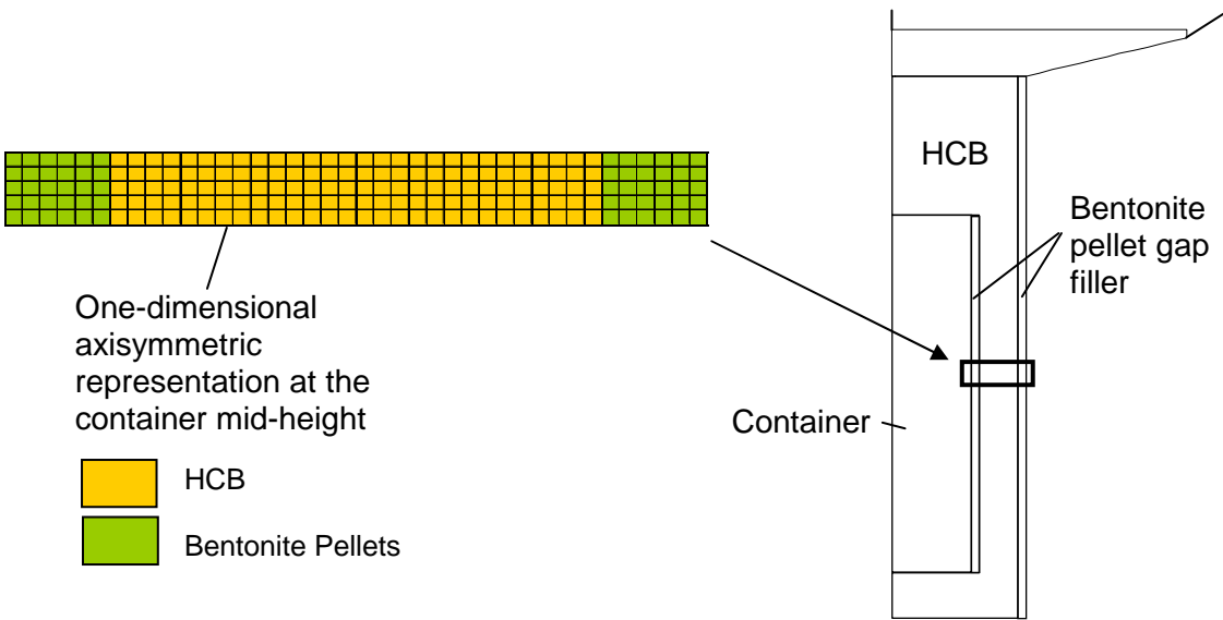
Figure 16: Simple One-dimensional and Two-dimensional Axisymmetric Representations used in Modelling.
