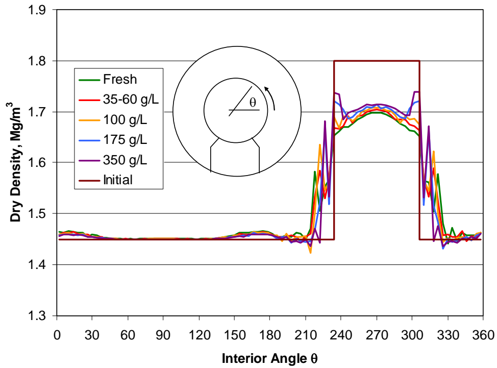
Figure B.5: Dry Density of the Bentonite Adjacent to the Container Surface for the Case of Initial Pellet Density of 1.45 \text{ Mg/m}^3 .
