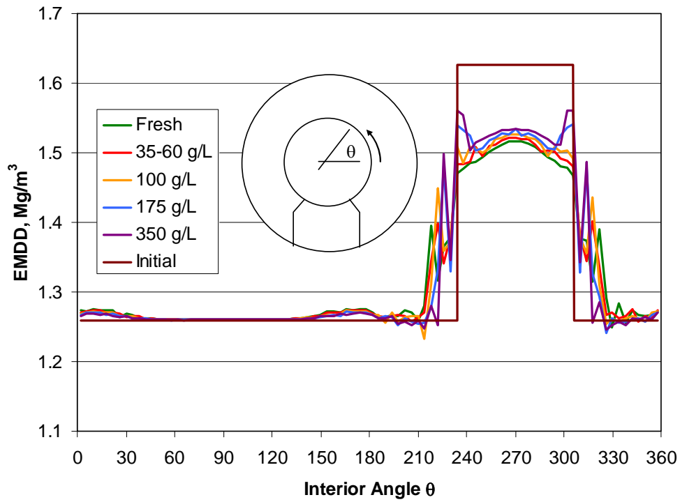
Figure B.6: EMDD of the Bentonite Adjacent to the Container Surface for the Case of Initial Pellet Density of 1.45 \text{ Mg/m}^3 .
