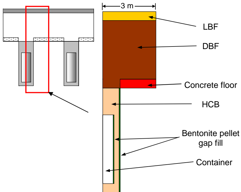
Figure 17: Configuration of Two-Dimensional Axisymmetric Model of the In-Floor Borehole Placement Design Option.
