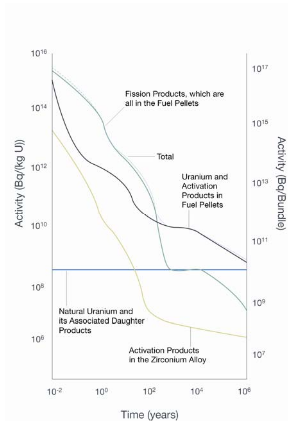
Figure 2: Total activity of used CANDU fuel as a function of time out of reactor. (Ref. DD1, p. 27)
