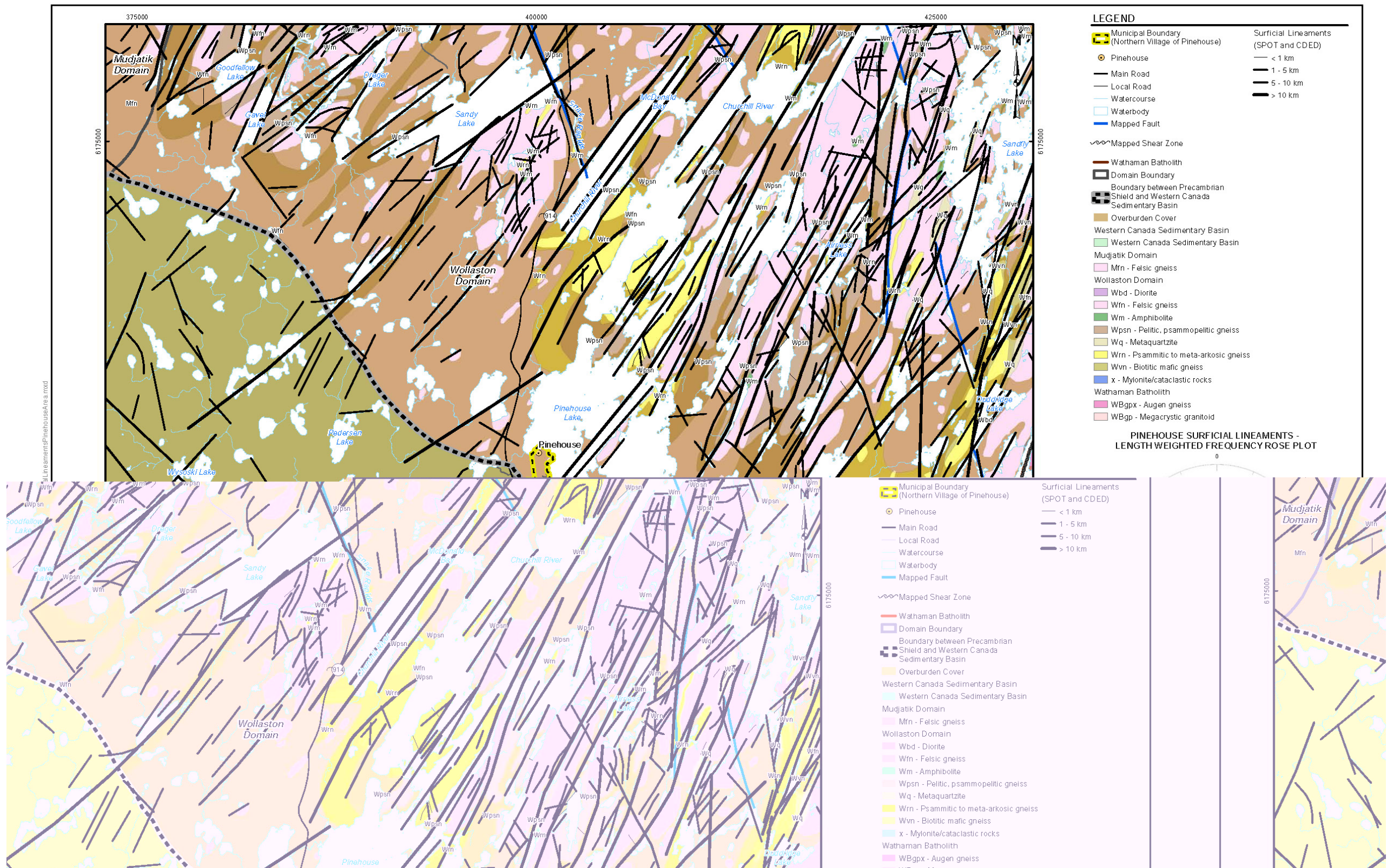
Figure 4-5: Surficial Lineaments of the Pinehouse Area
