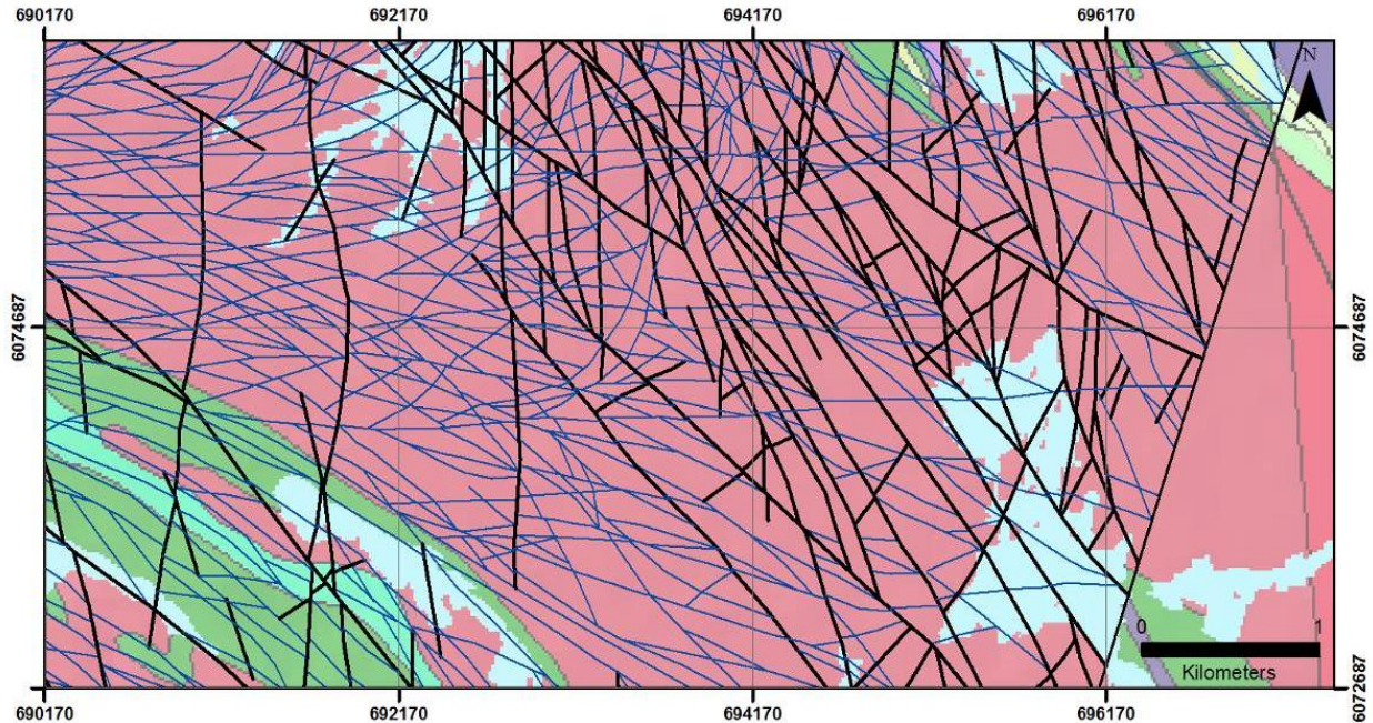
Figure A7: Within Final Integrated Lineaments, Corridor of Northwest-oriented D_5 - D_6 (brittle) Lineaments (black) Truncating and Offsetting Older D_2 - D_4 Brittle-ductile Lineaments (blue) Note a lower number of D_2 - D_4 brittle-ductile lineaments in the northwest-oriented D_5 - D_6 lineament corridor.
