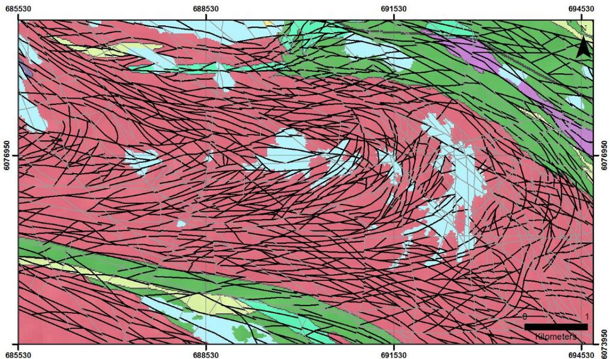
Figure A8: Within Final Integrated Lineaments, D_2 - D_4 Brittle-ductile Lineaments (black) Defining Hinge of Fold within the Annabel Lake Pluton Note tighter spacing of D_2 - D_4 lineaments in hinge of fold relative to surrounding areas. (Younger lineaments in grey).
