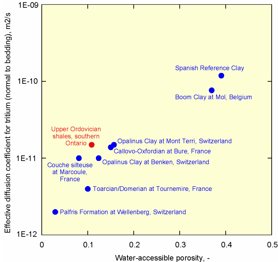
Figure 8-4: Water accessible porosity vs. effective diffusion coefficient for ^3\text{H} (values normal to bedding if specified in the original data) of various argillaceous formations compared with data of shales from southern Ontario. For shales from southern Ontario, the effective diffusion coefficient for \text{Cl}^- is shown (no data for ^3\text{H} available). Data taken from Table 8-3.
