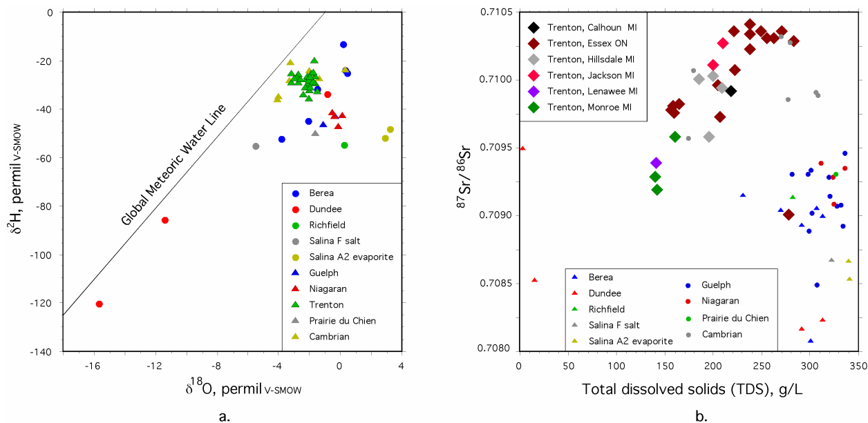
Figure 6-11: Chemical characteristics of formation waters from southwestern Ontario and Michigan (data from McNutt et al. 1987).
