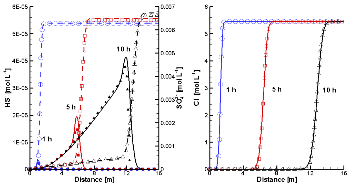
Figure 6: Comparison of Concentration Profiles of \text{HS}^- (Solid Lines/Filled Symbols) and \text{SO}_4^{2-} (Dashed Lines/Open Symbols) (Left) and Profiles of \text{Cl}^- (Right) at 1 (Blue), 5 (Red) and 10 (Black) Hours Simulated Using MIN3P-THCm (lines) to Those Simulated Using PHREEQC (Symbols)
