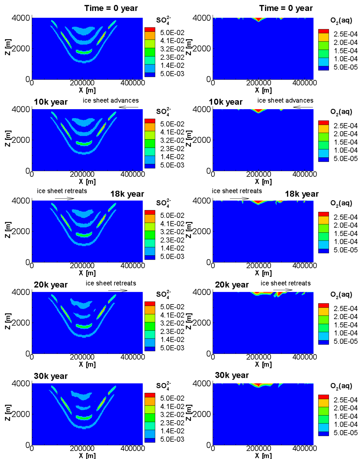
Figure 27: Simulated Concentration (in [\text{mol L}^{-1}] ) Contours of \text{SO}_4^{2-} (Left) and Dissolved \text{O}_2(\text{aq}) for the Case ELEVATED-SULPHATE – Glaciation/Deglaciation Scenario
