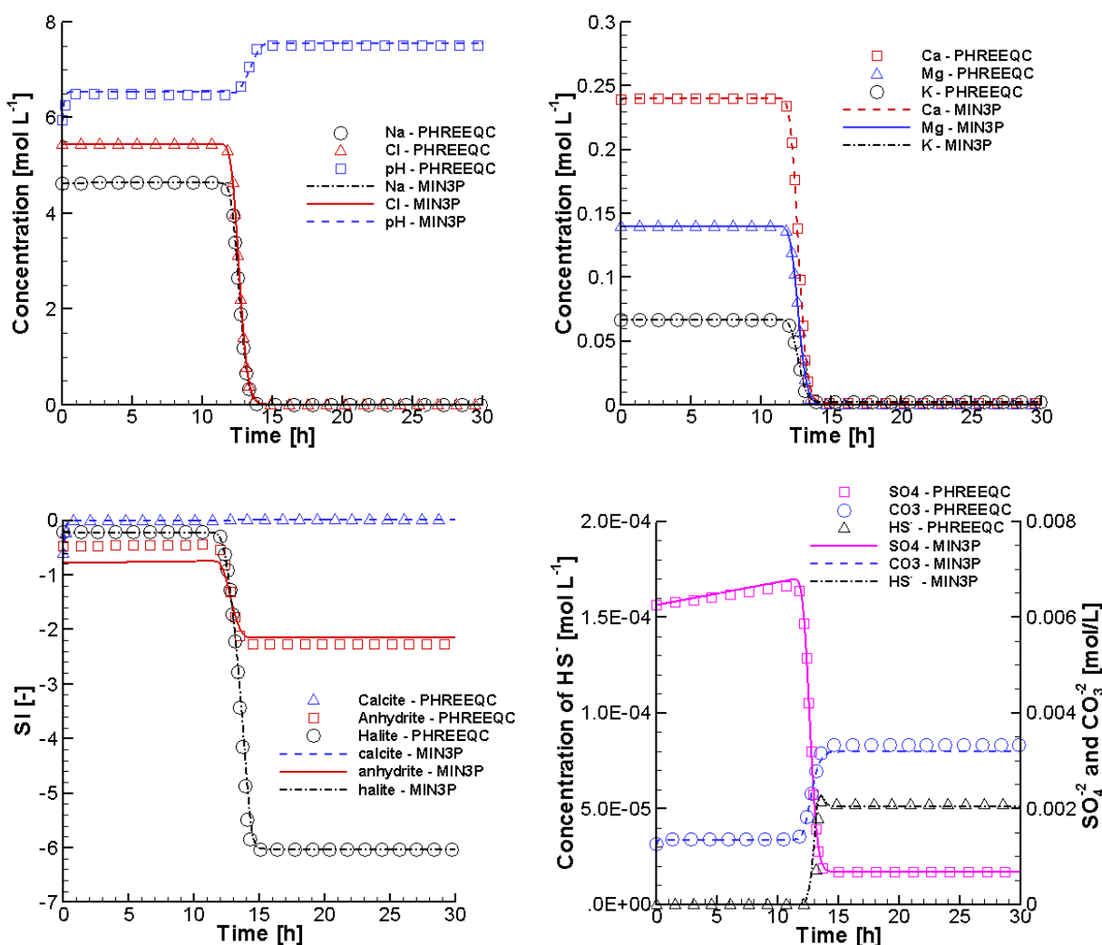
Figure 7: Comparison of Breakthrough Curves of pH and Total Concentrations of Na + and Cl - (Top Left), Mg 2+ , Ca 2+ , K + (Top Right), SO 4 2- , CO 3 2- and HS - (Bottom Right), and SI (saturation indexes) of Calcite, Anhydrite and Halite (Bottom Left) Simulated by MIN3P-THCm (Lines) to Those Calculated by PHREEQC (Symbols) – With Inhibition of Sulphate Reduction by Cl -
