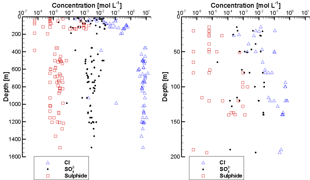
Figure 3: Measured Chloride, Sulphate and Sulphide Concentrations (in mol L -1 ) vs Sampling Depth. Left – Overview; Right – Detailed View from 0 to 200 m Depth (Based on Data Presented by Carter et al. 2015)
