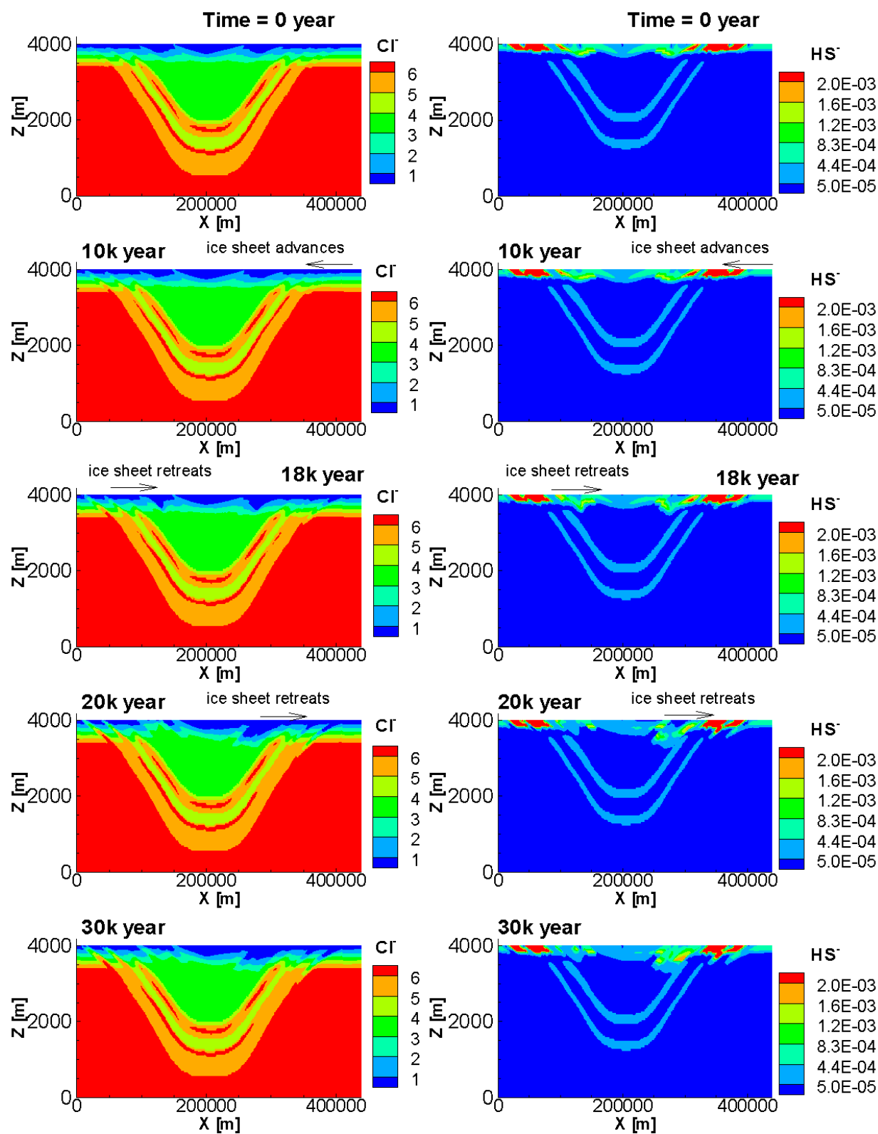
Figure 28: Simulated Contours of \text{Cl}^- and \text{HS}^- Concentrations (in [\text{mol L}^{-1}] ) for the Case ELEVATED-SULPHATE – Glaciation/Deglaciation Scenario
