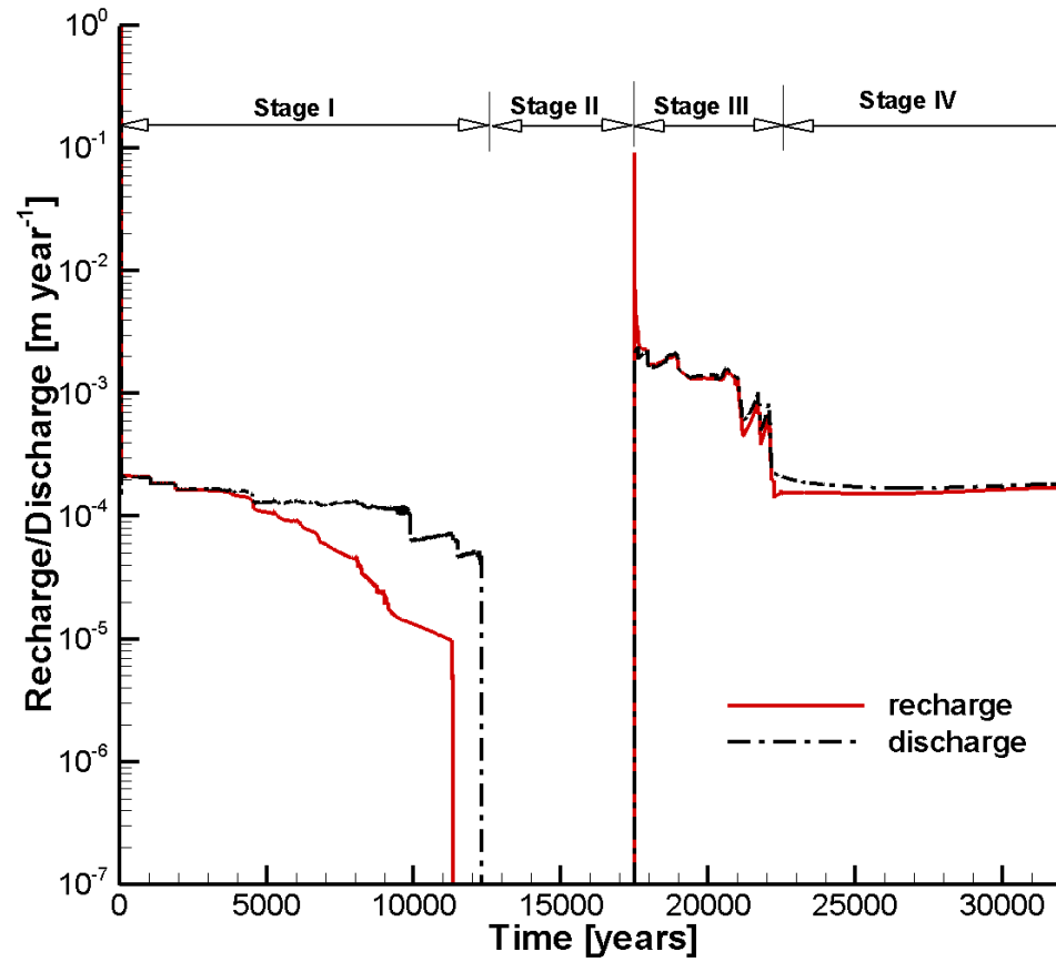
Figure 22: Simulated Temporal Evolution of Recharge and Discharge for the Case BASE – Glaciation/Deglaciation Scenario
