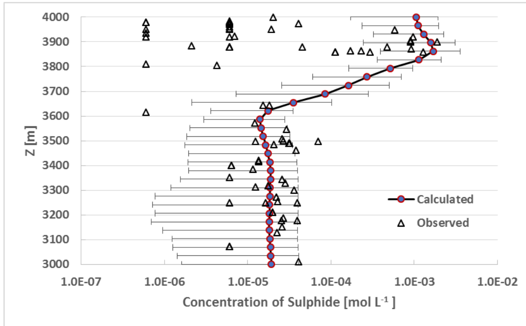
Figure 19: Comparison of the Observed Sulphide Data and the Simulated Average \text{HS}^- Concentrations (in [\text{mol L}^{-1}] ) \pm Standard Deviations (Horizontal Black Lines) at Different Depths for the Region Shown in Figure 18(g). Simulation Results are for the Case ELEVATED-SULPHATE at 3.25 \times 10^4 Years under Interglacial Conditions; Observed Data are from Carter et al. (2015)
