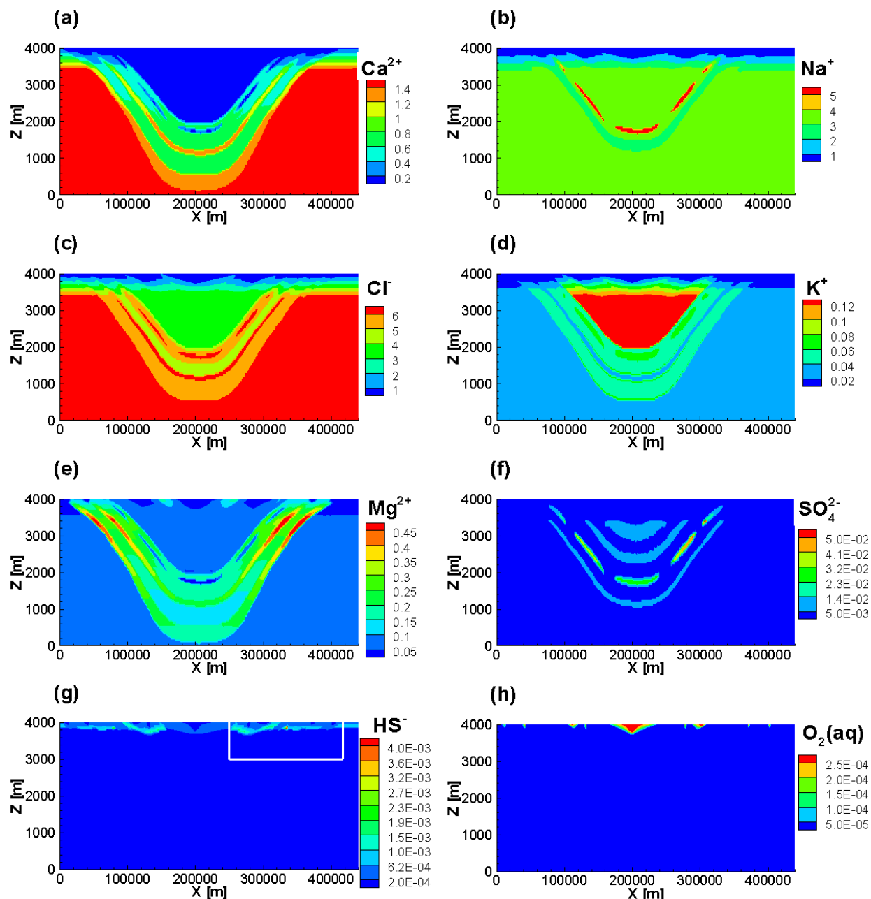
Figure 16: Total Concentration Contours (in \text{mol L}^{-1} ) of Chemical Components for the case BASE at 3.25 \times 10^4 Years. White Rectangle Indicates the Data Extraction Region (i.e. Horizontal Extent from 250 to 420 km and Vertical Extent from 3000 to 4000 m) for \text{HS}^- Concentrations Shown in Figure 17
