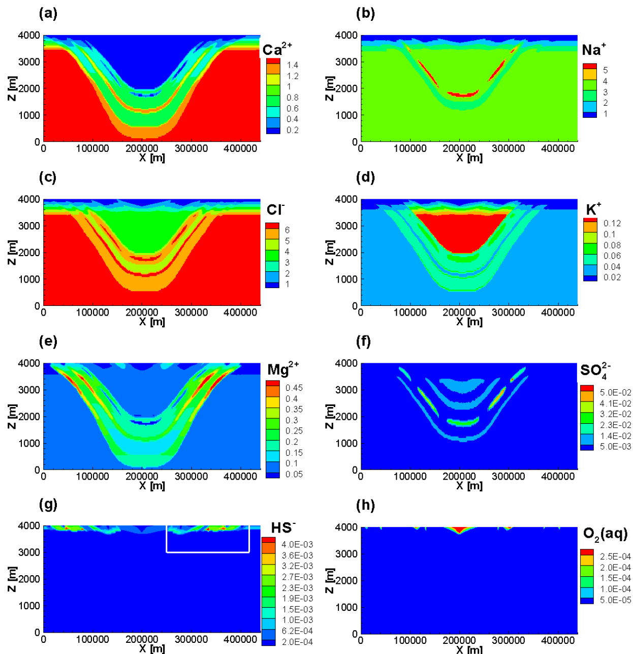
Figure 18: Total Concentration Contours of Chemical Components (in \text{mol L}^{-1} ) for the Case ELEVATED-SULPHATE at 3.25 \times 10^4 Years. The White Rectangle in (g) Indicates the Data Extraction Region (i.e. Horizontal from 250 to 420 km and Vertical from 3000 to 4000 m) for \text{HS}^- Concentrations Shown in Figure 19
