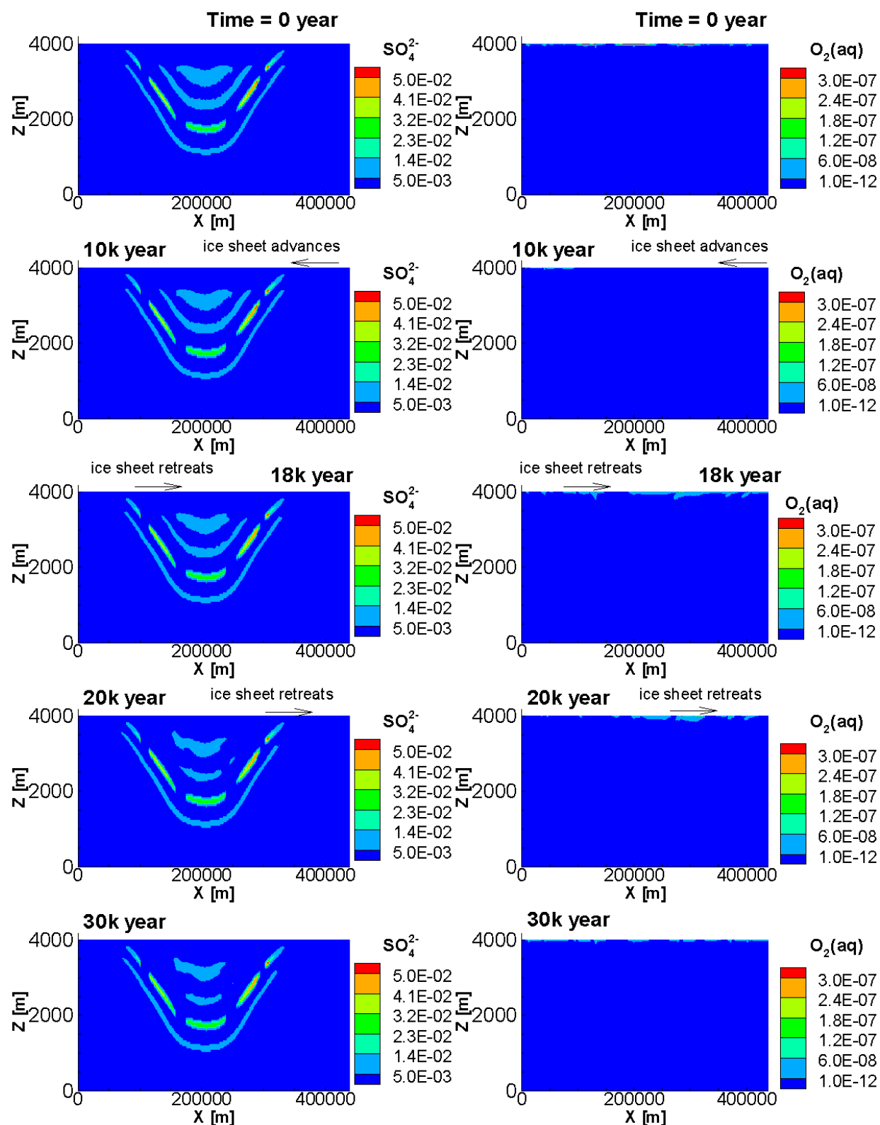
Figure 30: Simulated Contours of \text{SO}_4^{2-} and \text{O}_2(\text{aq}) Concentrations (in \text{mol L}^{-1} ) for the Case OXYGEN-CONSUMPTION – Glaciation/Deglaciation Scenario
