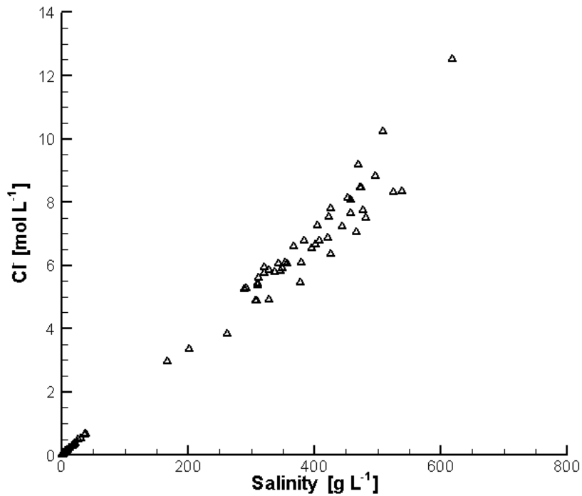
Figure 5: Correlation of Salinity and \text{Cl}^- Concentration in Southern Ontario Groundwaters (Based on Data Presented by Carter et al. 2015)
