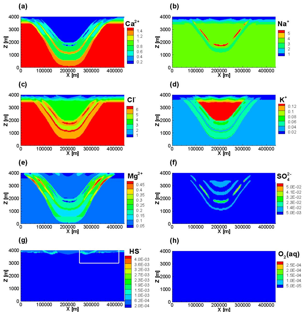
Figure 20: Total Concentration Contours of Chemical Components (in \text{mol L}^{-1} ) for the Case OXYGEN-CONSUMPTION at 3.25 \times 10^4 Years. The White Rectangle Indicates the Data Extraction Region (i.e. Horizontal Extension from 250 to 420 km and Vertical Extension from 3000 to 4000 m) for \text{HS}^- Concentrations Shown in Figure 21
