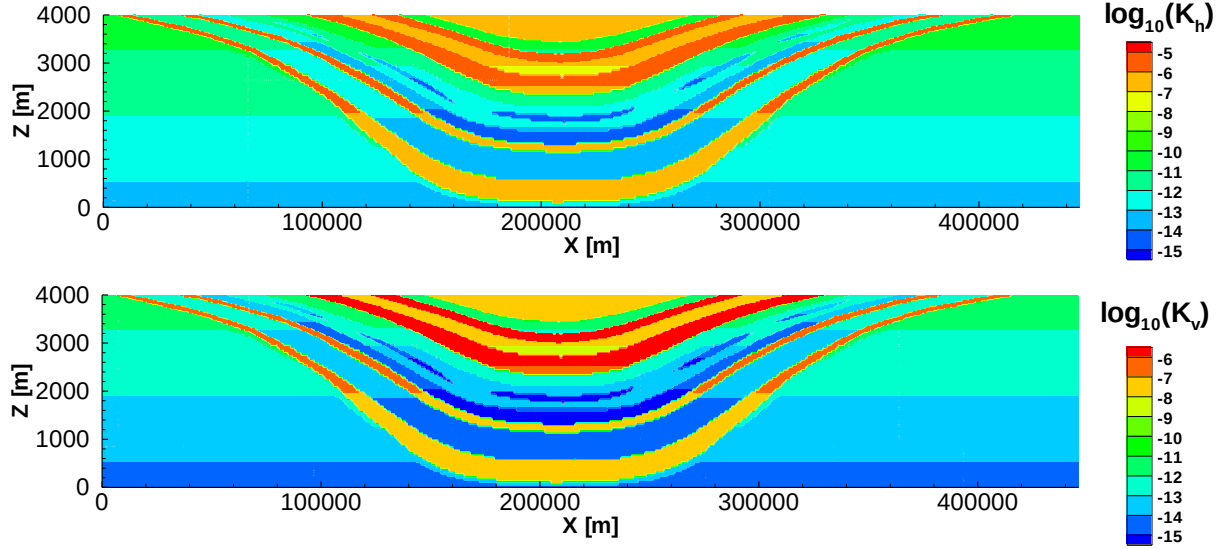
Figure 11: Profiles of Initial Horizontal (Upper Panel) and Vertical (Lower Panel) Hydraulic Conductivities (in \log_{10}[\text{m s}^{-1}] )
