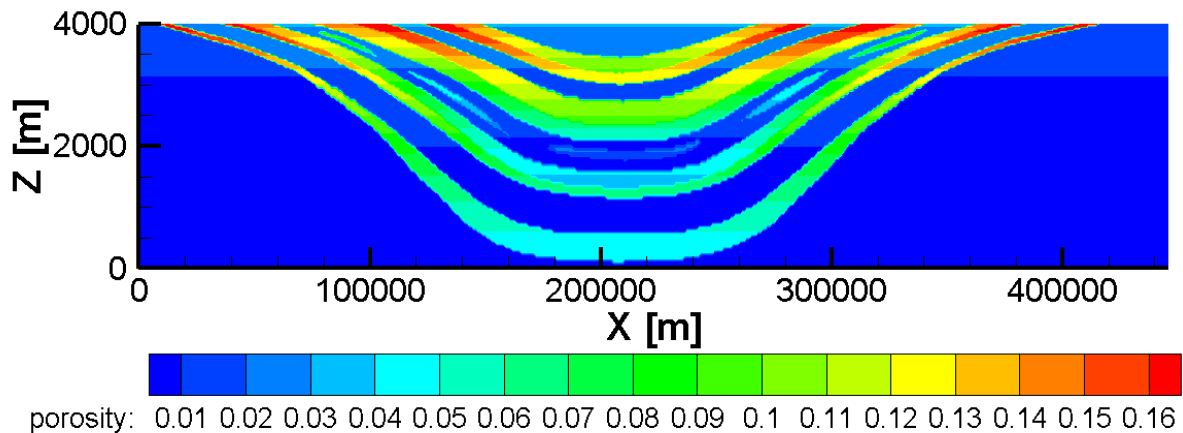
Figure 10: Distribution of Initial Porosity (According to Bea et al. 2011)
