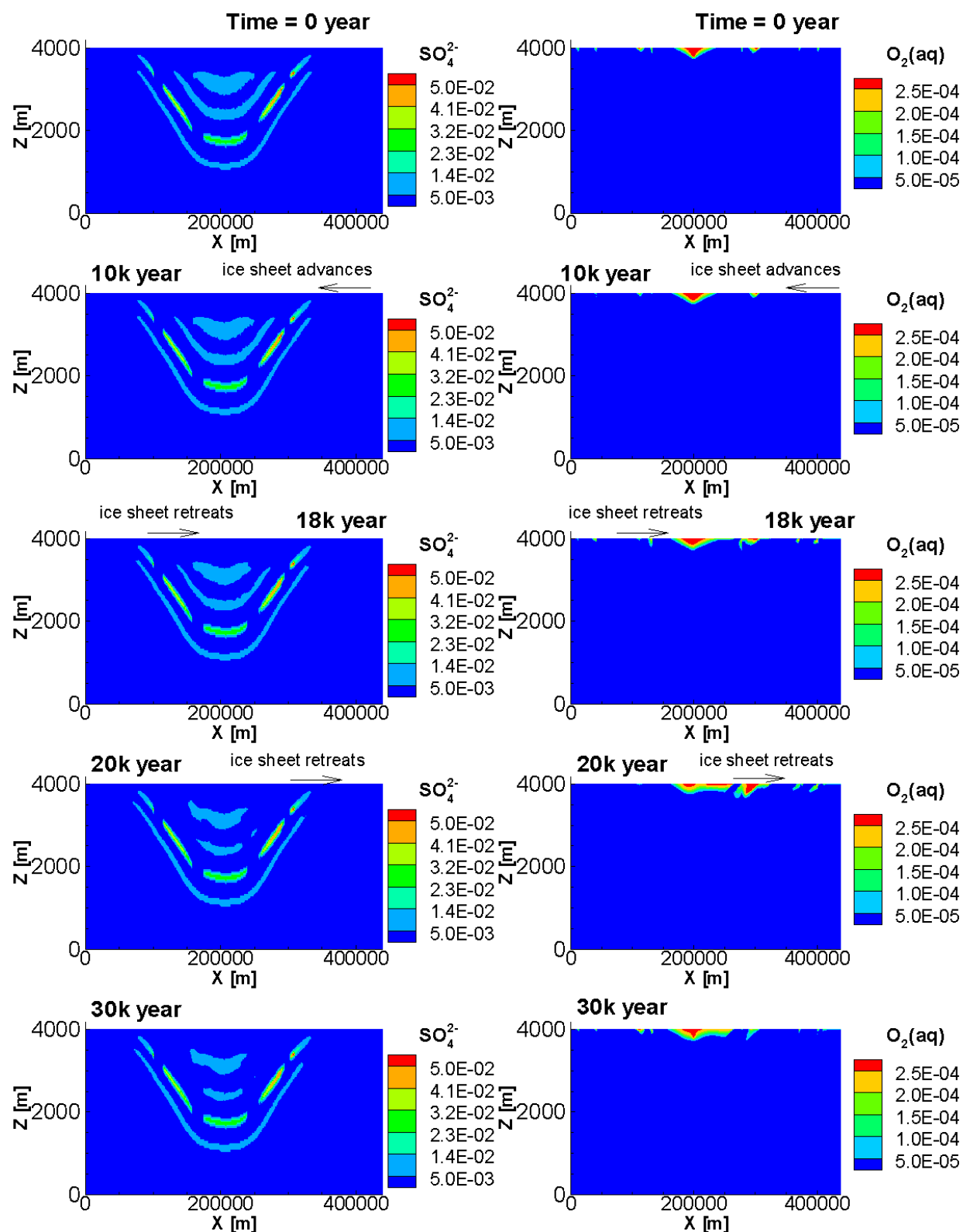
Figure 24: Simulated Contours of \text{SO}_4^{2-} and Dissolved \text{O}_2(\text{aq}) Concentrations (in \text{mol L}^{-1} ) for the Case BASE – Glaciation/Deglaciation Scenario
