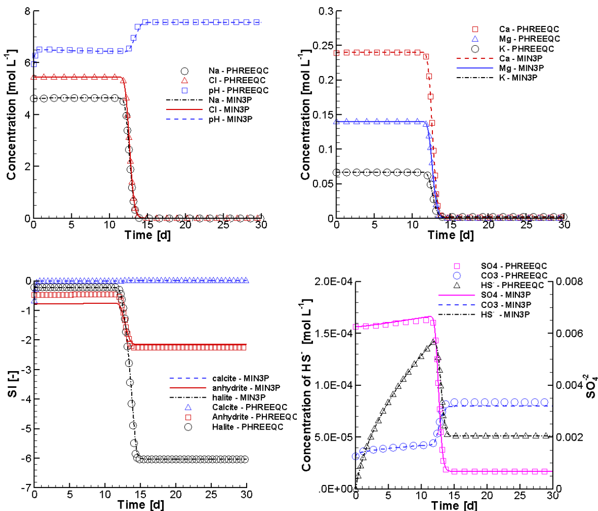
Figure 8: Comparison of Breakthrough Curves of pH and Total Concentrations of Na + and Cl - (Top Left), Ca 2+ , K + , Mg 2+ (Top Right), SO 4 2- , CO 3 2- and HS - (Bottom Right), and SI (saturation indexes) of Calcite, Anhydrite and Halite (Bottom Left) Simulated by MIN3P-THCm (Lines) to Those Calculated by PHREEQC (Symbols) – Without Inhibition of Sulphate Reduction by Cl -
