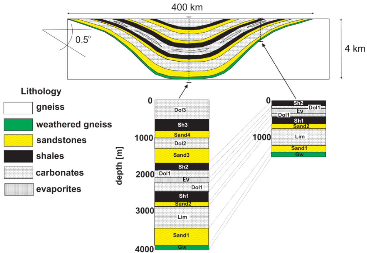
Figure 9: Geometry and Main Hydrogeological Units Considered (Bea et al. 2011)
