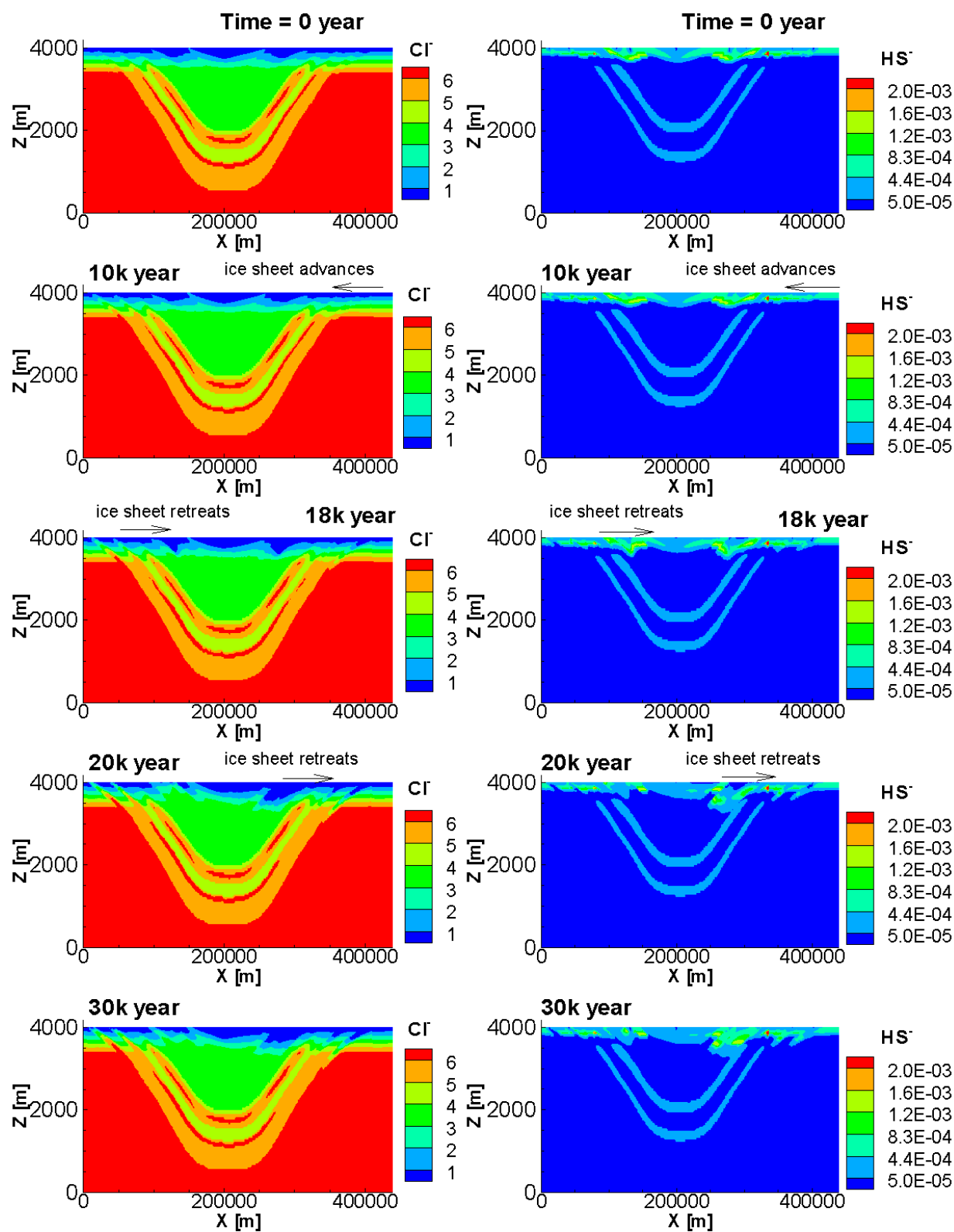
Figure 25: Simulated Contours of \text{Cl}^- and \text{HS}^- Concentrations (in \text{mol L}^{-1} ) for the Case BASE – Glaciation/Deglaciation Scenario
