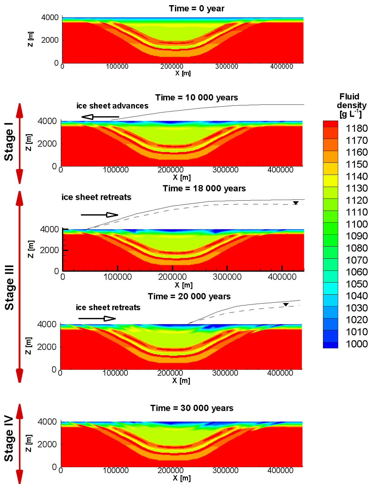
Figure 23: Simulated Liquid Phase Density for the Case BASE – Glaciation/Deglaciation Scenario
