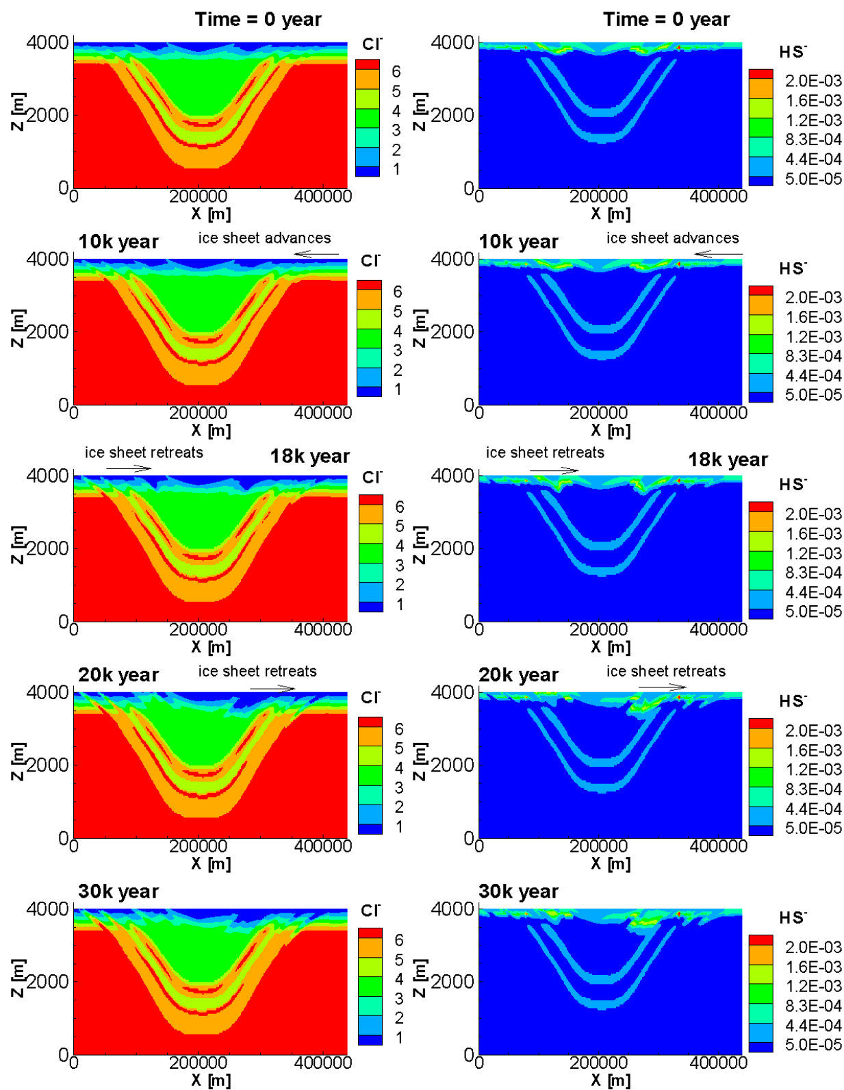
Figure 29: Simulated Contours of \text{Cl}^- and \text{HS}^- Concentrations (in \text{mol L}^{-1} ) for the Case OXYGEN-CONSUMPTION – Glaciation/Deglaciation Scenario
