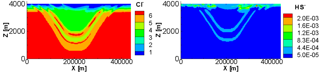
Figure 26: Concentration Contours of \text{Cl}^- (left) and \text{HS}^- (right) (in [\text{mol L}^{-1}] ) for the case BASE at 50,000 Years
