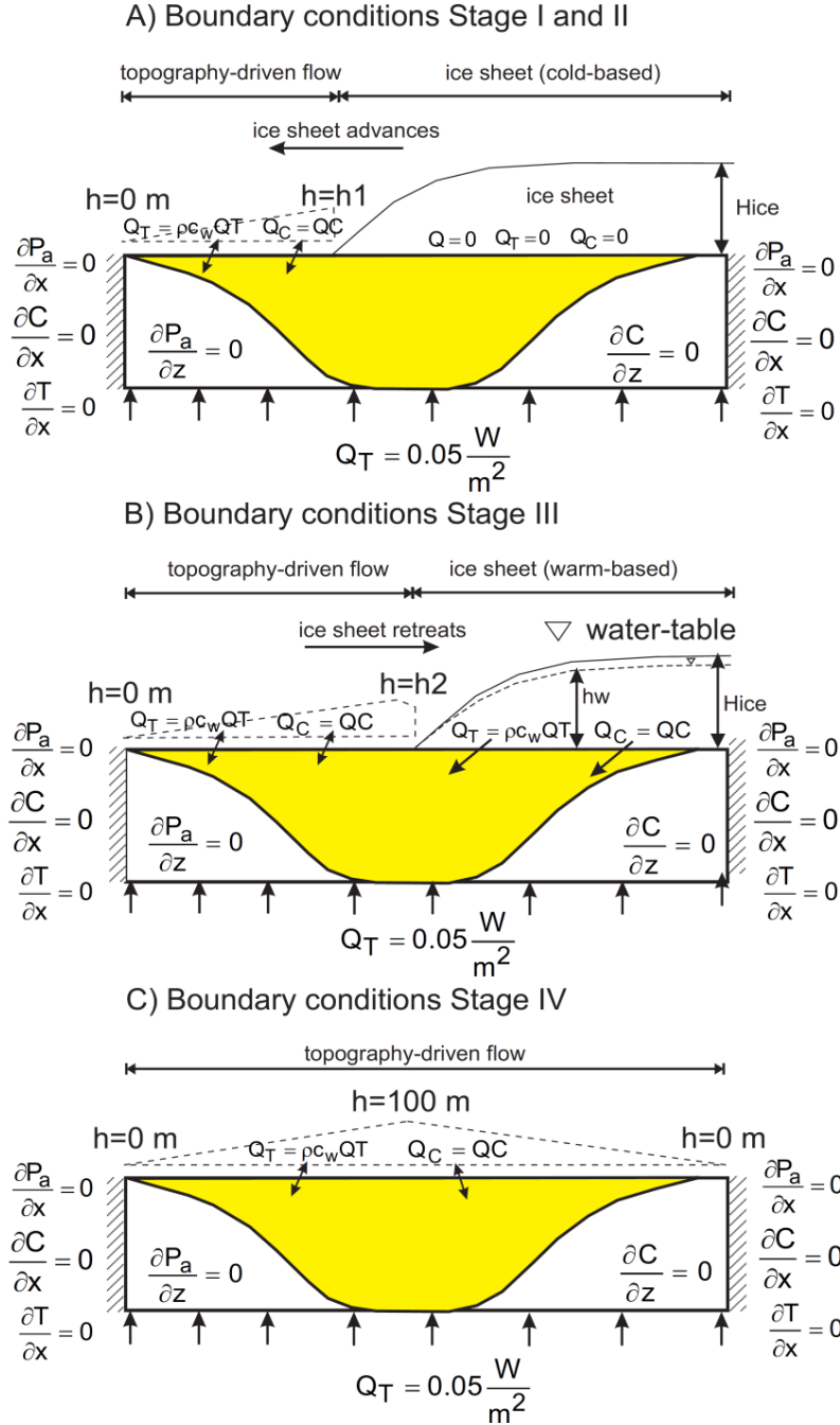
Figure 13: Boundary Conditions Imposed in the Simulations: A) Stage I (i.e. Ice Sheet Accumulation) and Stage II (i.e. Constant Ice Sheet Thickness). B) Stage III (i.e. Ice Sheet Retreat). C) No Ice Present (i.e. Present Day Conditions). Q is the Volumetric Recharge or Discharge per Unit Area, Q_c is the Solute Mass Flux per Unit Area, C is Solute Concentration, h is the Hydraulic Head in Ice-Free Areas, H_{ice} is the Maximum Ice Sheet Thickness, and h_w is the Hydraulic Head beneath the Ice Sheet. Q_T is the Energy Flux per Unit Area, T is the Water Temperature, and c_w is the Specific Heat Capacity of Water (Bea et al. 2011)
