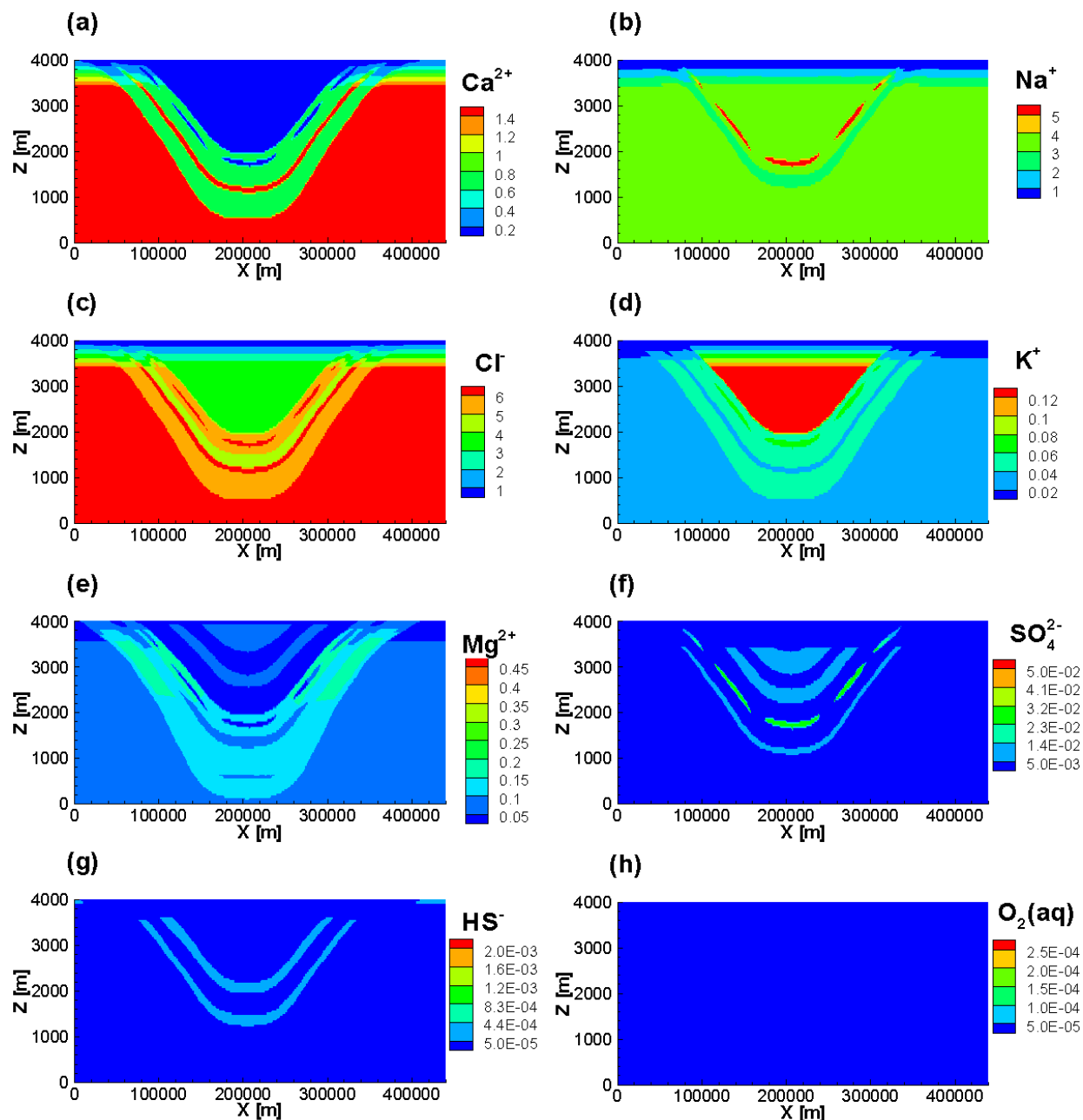
Figure 14: Initial Total Concentrations of Chemical Components for the Case BASE (in \text{mol L}^{-1} )
