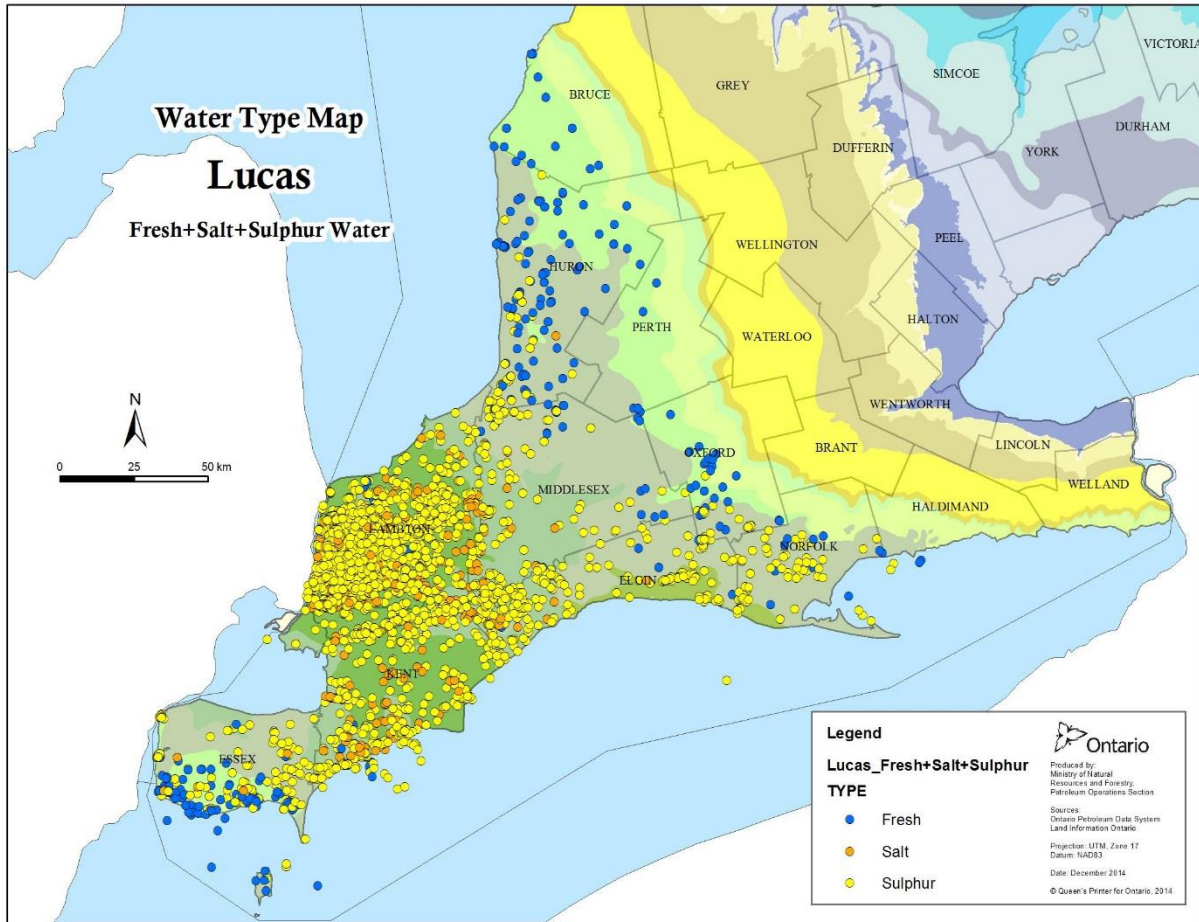
Figure 2: Water Type Map in the Lucas Formation in Southern Ontario (Carter et al. 2015)
