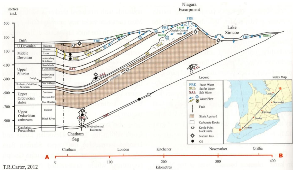
Figure 1: Conceptual Model and Observed Distribution of Sulphidic Water (SUL) at the Eastern Flank of the Michigan Basin (Carter 2012)
