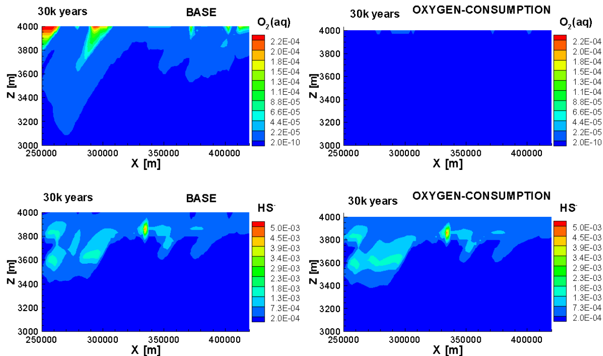
Figure 31: Comparison of Concentration (in [mol L -1 ]) Contours of O 2 (aq) and HS - for Case BASE (Left) and Case OXYGEN-CONSUMPTION (Right) for the Selected Region Shown in Figure 18(g) – Glaciation/Deglaciation Scenario
