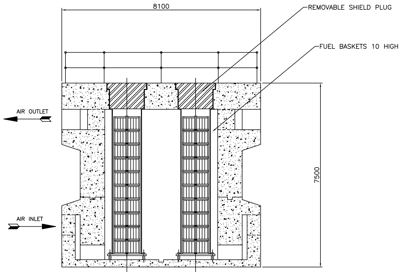
SECTION 'A'-'A' FROM FIGURES 6 & 7
