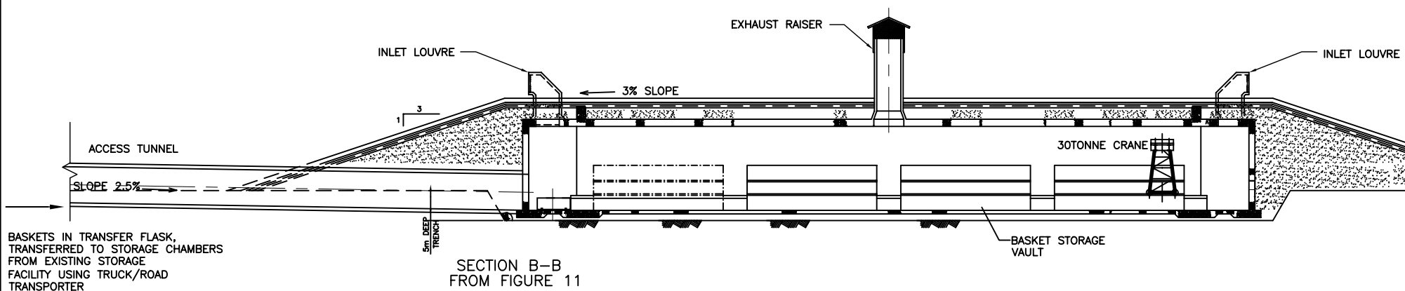
FIGURE 12 VAULTS IN A SHALLOW TRENCH STORAGE CHAMBERS – SECTIONS HYDRO-QUÉBEC GENTILLY REACTOR SITE
