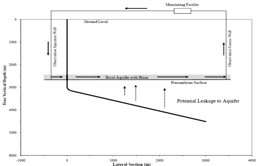
Figure 3: Brine circulation-loop in the basal aquifer to monitor leakage into the geosphere
