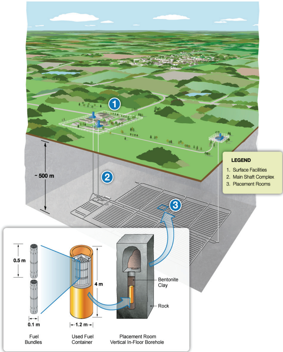
Figure 1: APM Deep Geological Repository in Crystalline Rock
