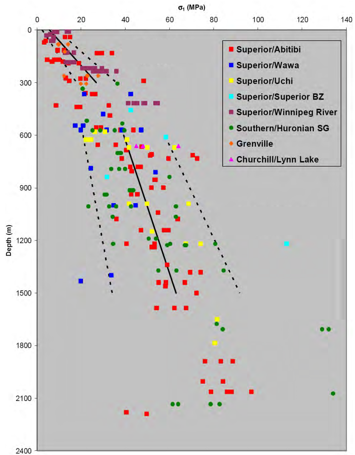
Maximum Horizontal In Situ Stresses Measured in the Canadian Shield
