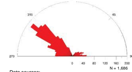
Dyke - Length Weighted Frequency Rose Plot
