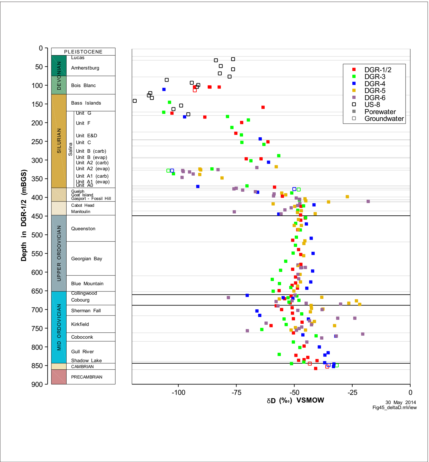
b. Deuterium (after Intera Engineering Ltd., 2011)
