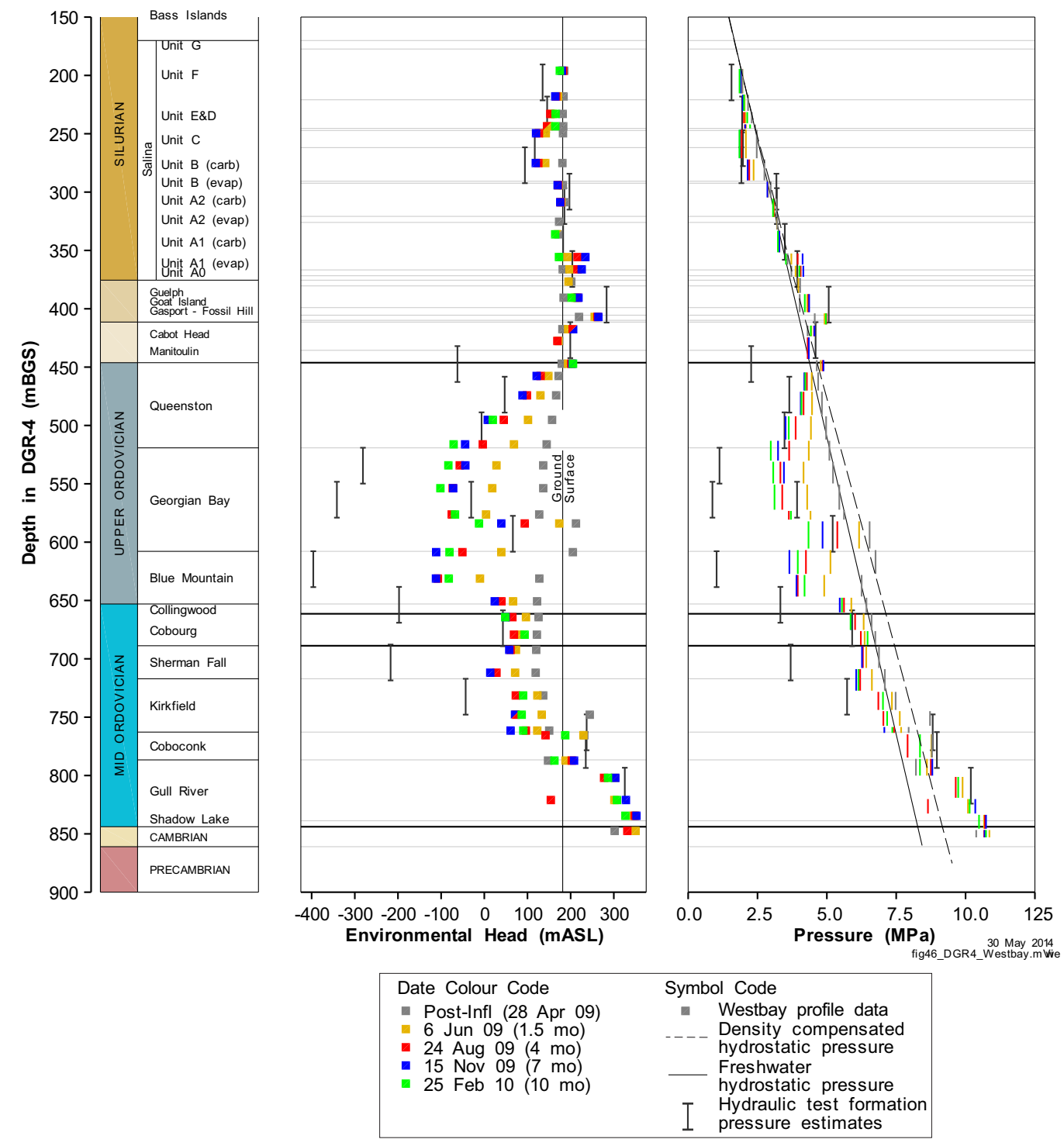
b. DGR-4 (after Intera Engineering Ltd., 2011)
