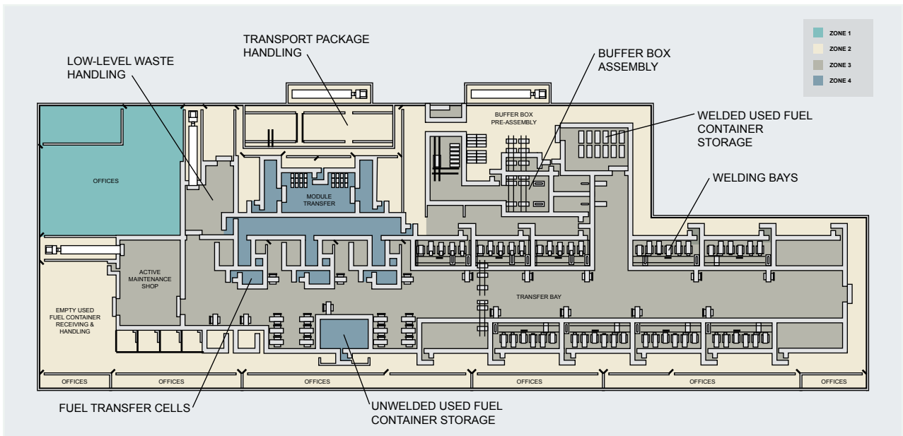
Example of a Layout for a UFPP
