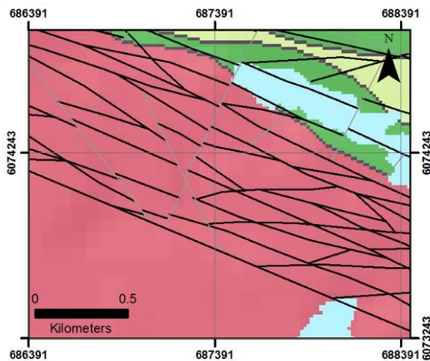
Figure A6: Final Integrated Continuous Northwest-oriented D_2 - D_4 Lineaments and Short East-West to East-northeast Secondary and Tertiary Linking D_2 - D_4 Shear Zones (black) (Younger lineaments in grey).
