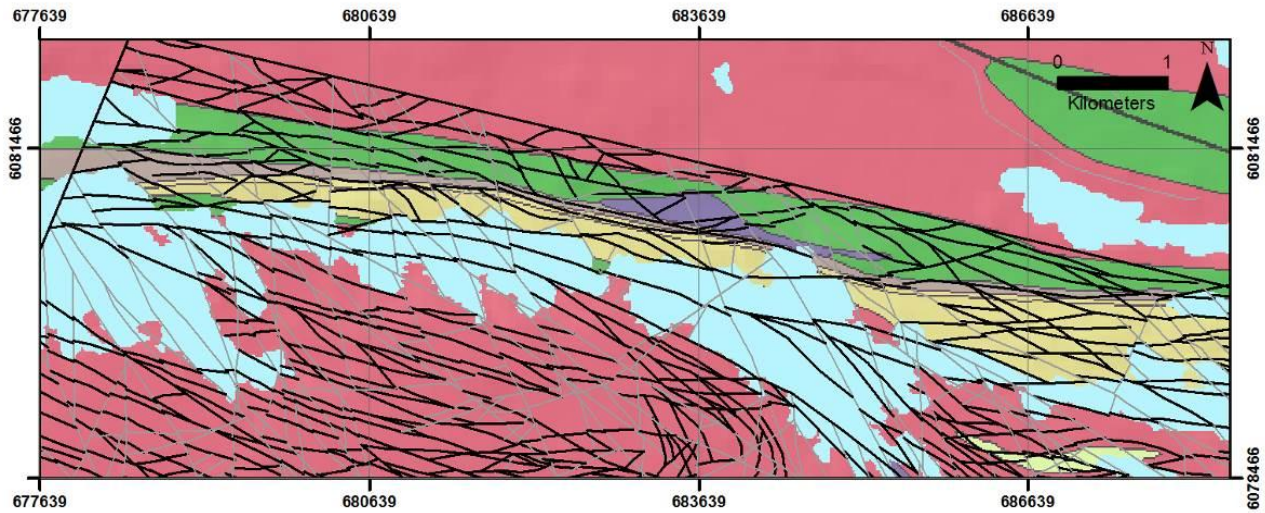
Figure A5: Final Integrated West-northwest Trending D_2 - D_4 Lineaments (black) Defining Orientation of Greenstone Belt (green), Metasedimentary Rocks (yellow) and Internal Geometry of Annabel Lake Pluton (red)
