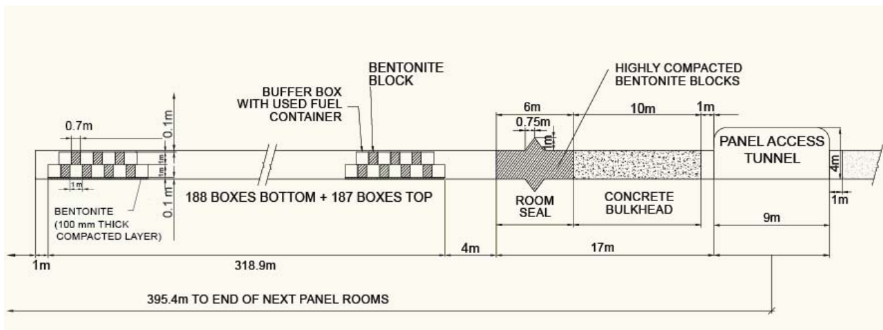
Figure 3: Conceptual Layout of Filled Emplacement Room
