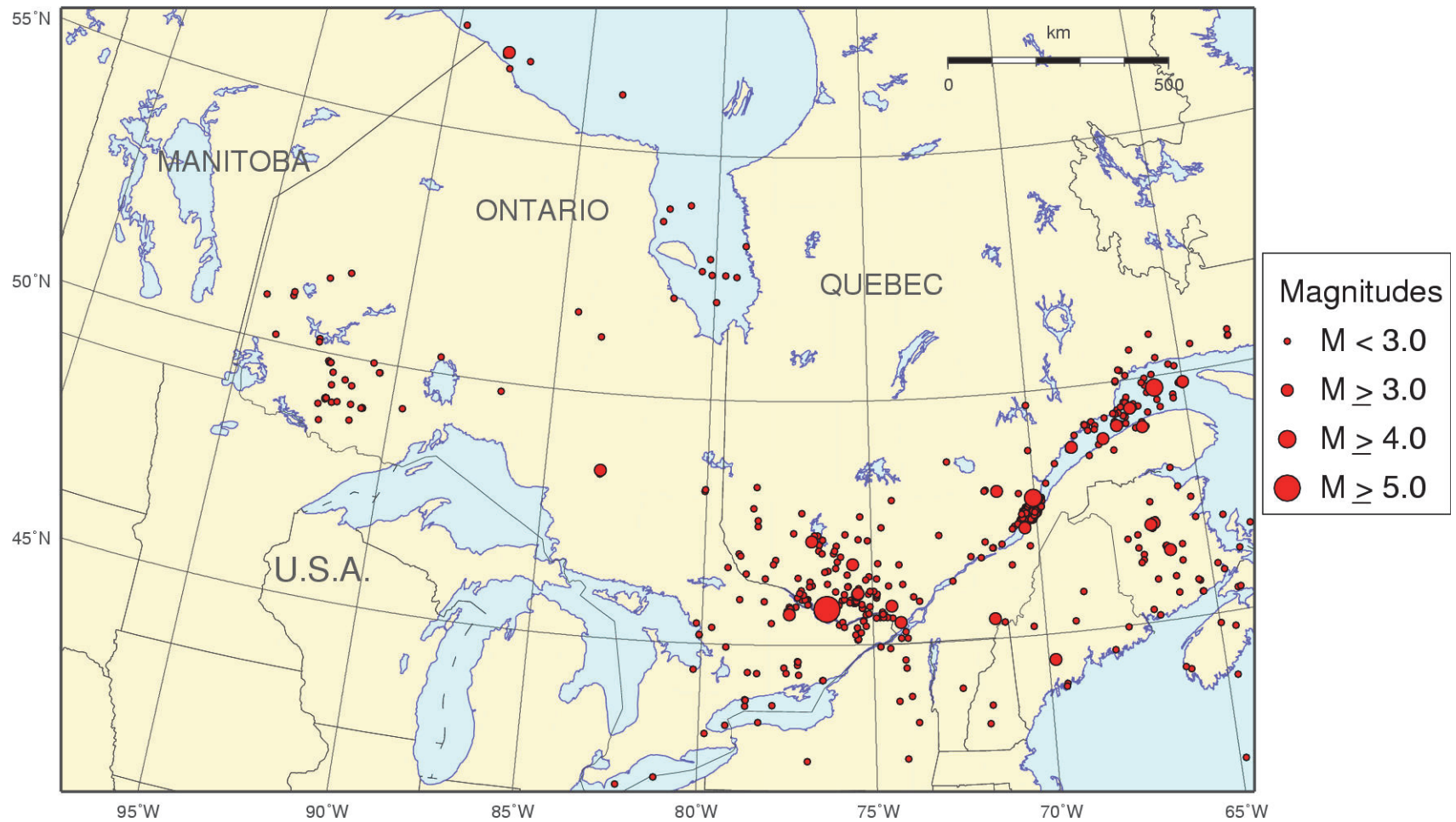
Figure 4: Earthquakes in Eastern Canada, 2013
