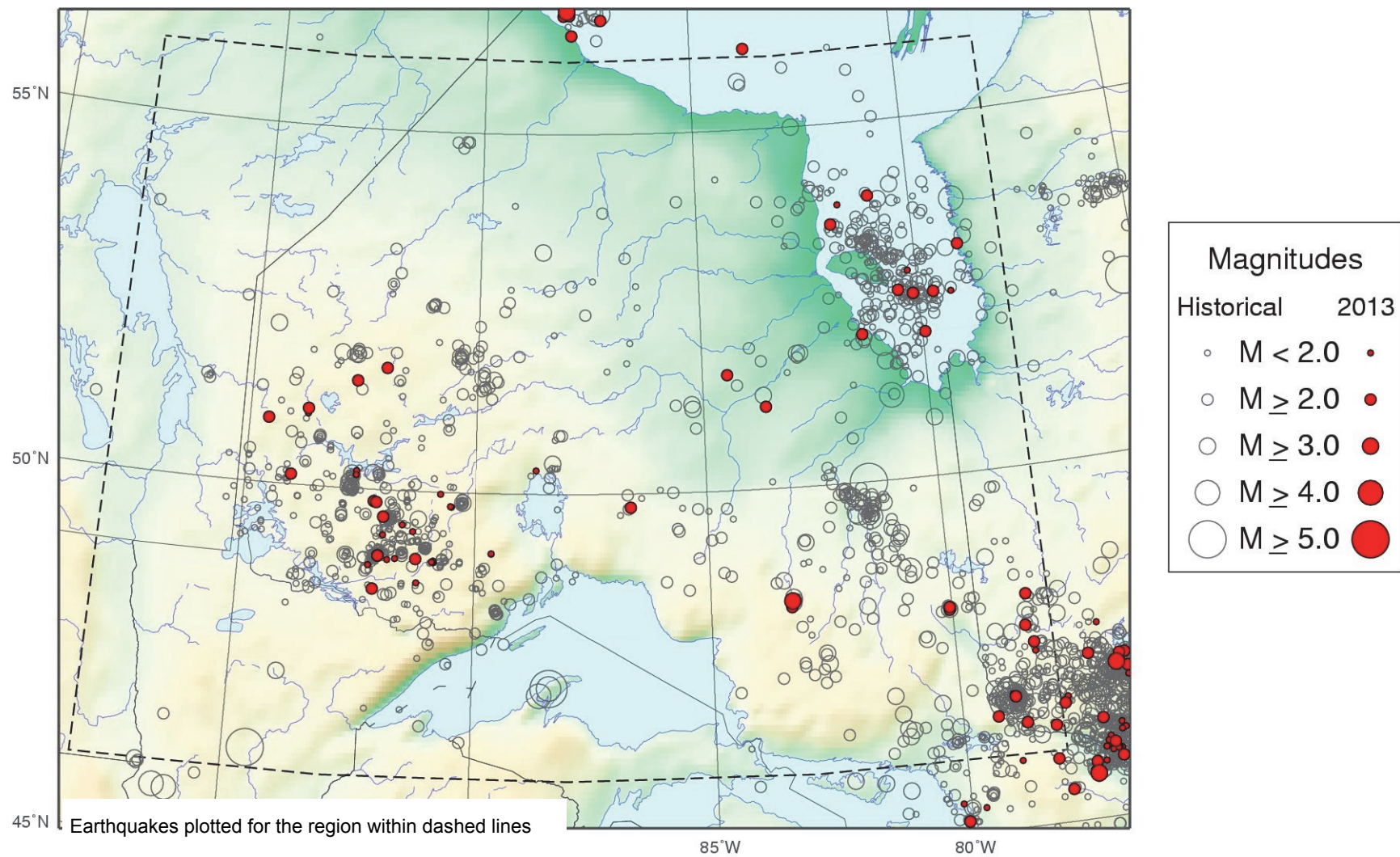
Figure 7: Earthquakes in Northern Ontario and Adjacent Areas for 2013 and prior years
