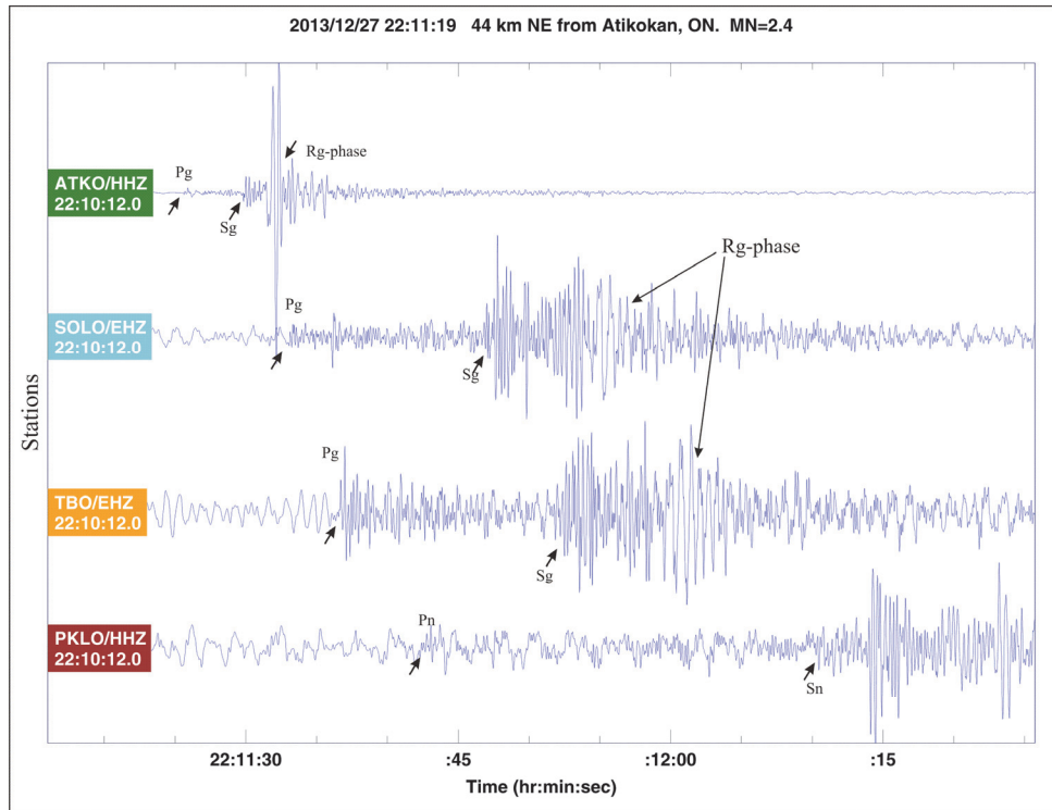
Figure 8: Rg Surface Waves from the m_N 2.4 on 2013/12/27, 44 km NE of Atikokan, ON
