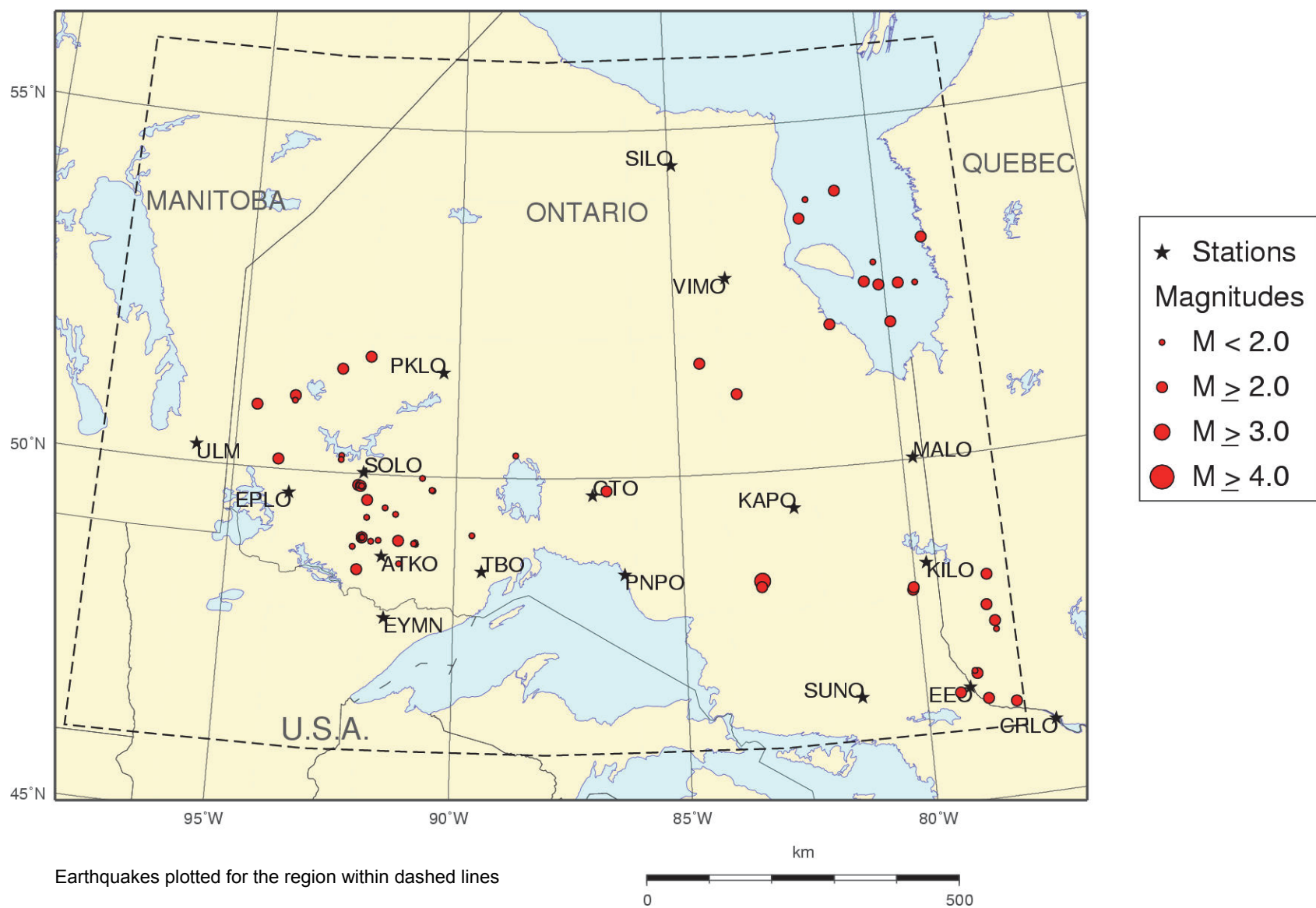
Figure 1: Earthquakes in Northern Ontario and Adjacent Areas, 2013
