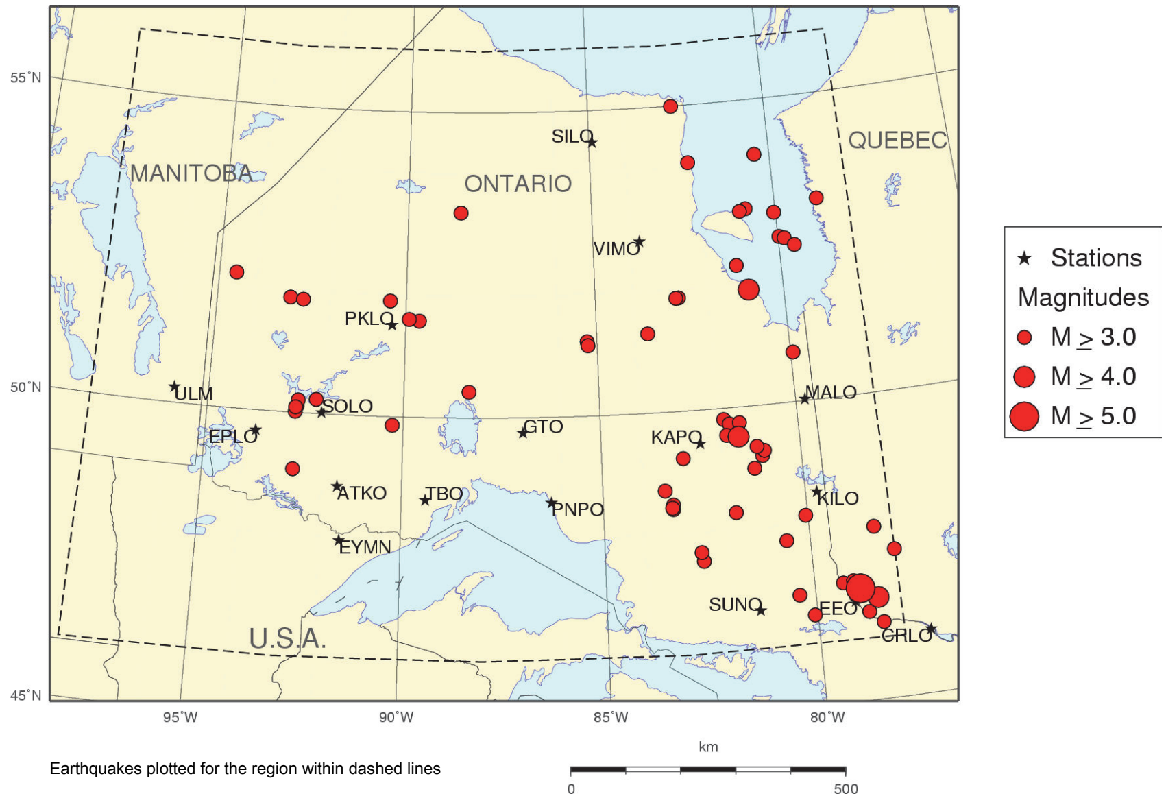
Figure 3: Earthquakes m_N \geq 3 in Northern Ontario and Adjacent Areas, 1982 – 2013
