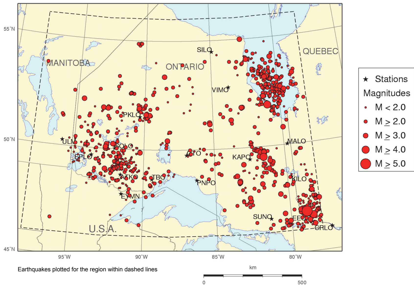
Figure 2: Earthquakes in Northern Ontario and Adjacent Areas, 1982 - 2013
