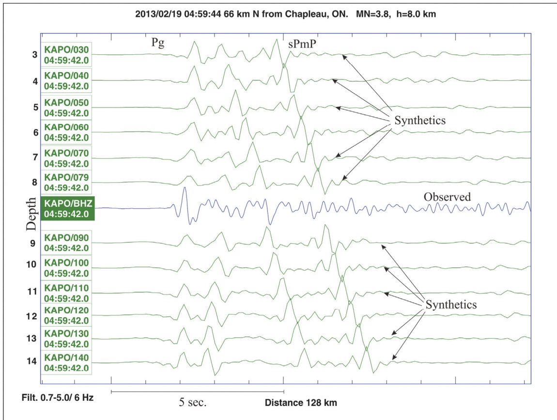
Figure 9: Observed and Synthetic Waveforms from the m_N 3.8 on 2013/02/19, 66 km north of Chapleau, ON
