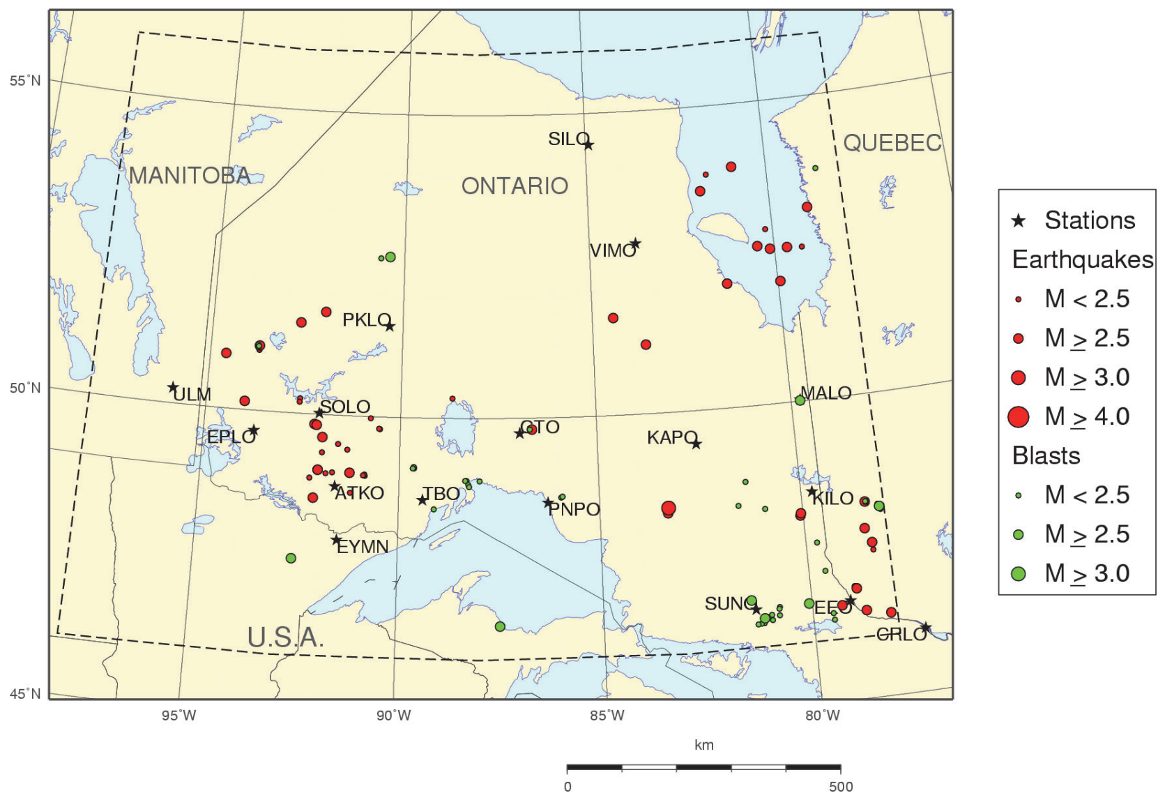
Figure 6: Earthquakes and Blasts in Northern Ontario and Adjacent Areas, 2013
