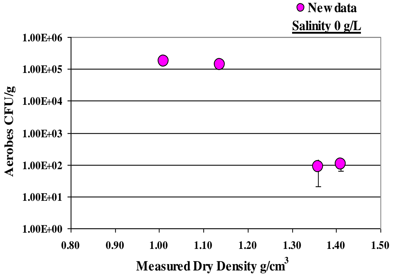
Figure 1: Aerobic culturability in compacted bentonite as a function of measured intermediate dry densities (target 1.1-1.5 g/cm 3 ) at a porewater salinity of 0 g NaCl/L
