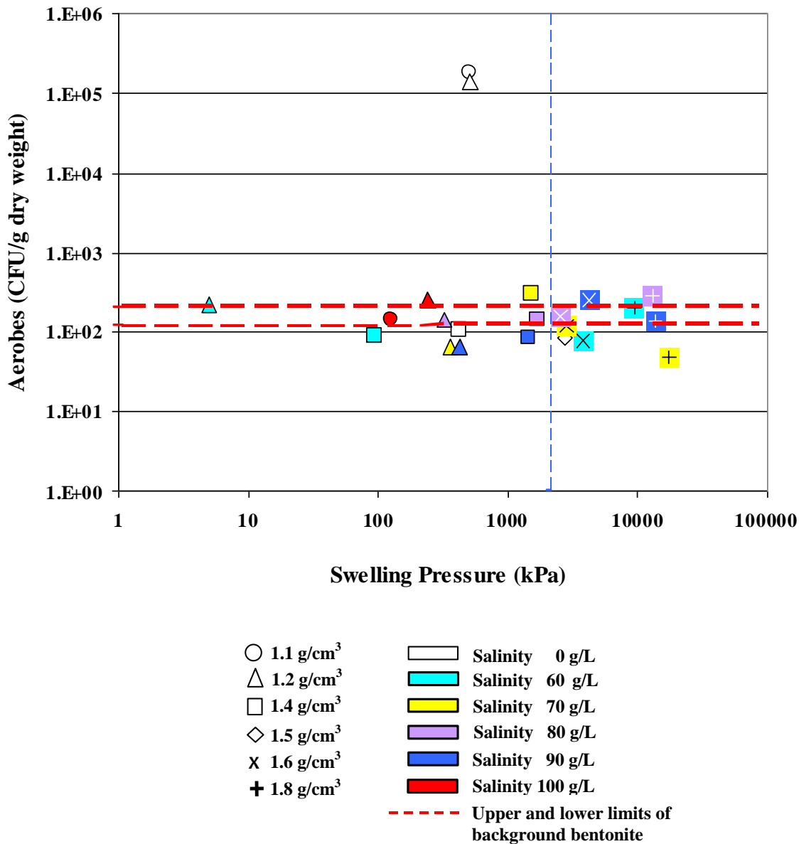
Figure 30: Aerobic culturability in compacted bentonite as a function of swelling pressure (new data).
